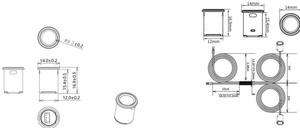
Dimension Diagram unit: mm
