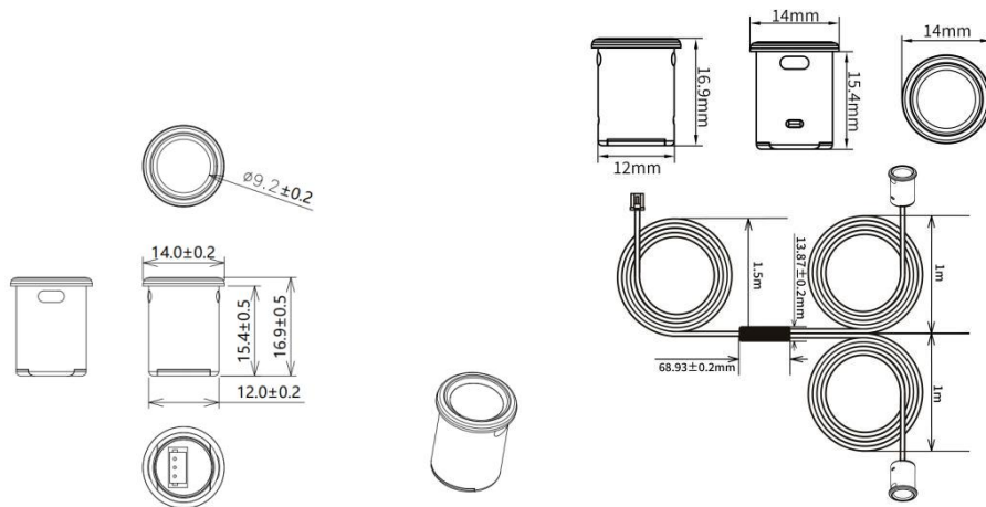
Dimension Diagram unit: mm
