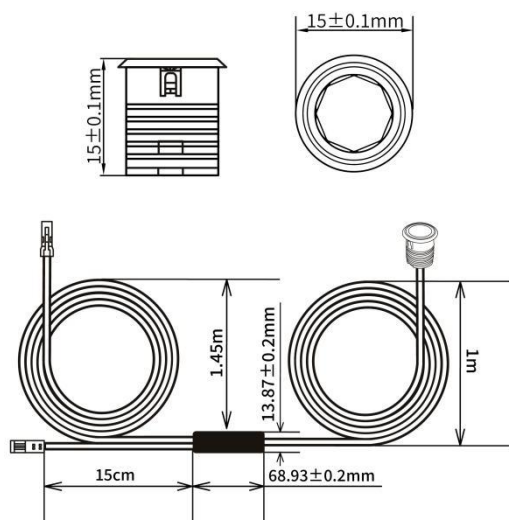
Dimension Diagram unit: mm
