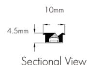
Sectional View
